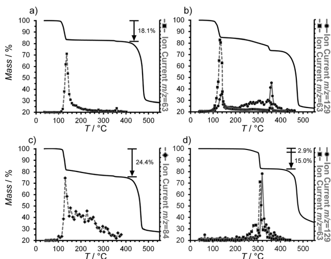
Figure 2. Tandem TGA-MS analysis of phase-pure crystal forms of 111 : a) triclinic 0.5 H 2 O@ 111 ·1.5 DCE, b) isostructural 0.73 Xe@ 111 ·1.5 DCE, c) isostructural 0.80 Kr@ 111 ·1.5 DCE, and d) trigonal Xe@ 111 ·0.2 DCE. TGA curves are in black, whereas the curves with markers represent the MS ion current (arbitrary units) of guests (vinyl chloride, m/z = 63 ; xenon, m/z = 129 ; krypton m/z = 84 ).
